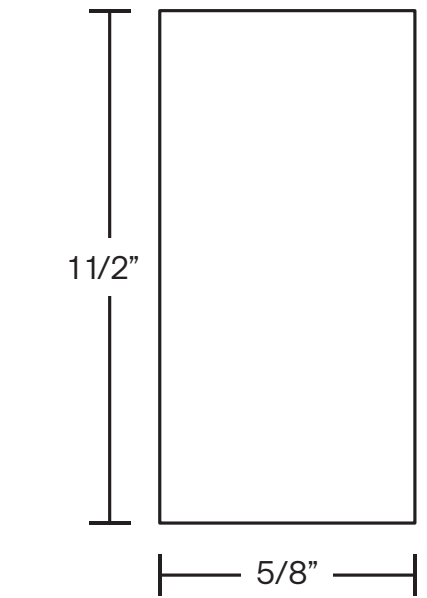
DM/SHA90 Shade Moulding (Melamine on Particle Board)
