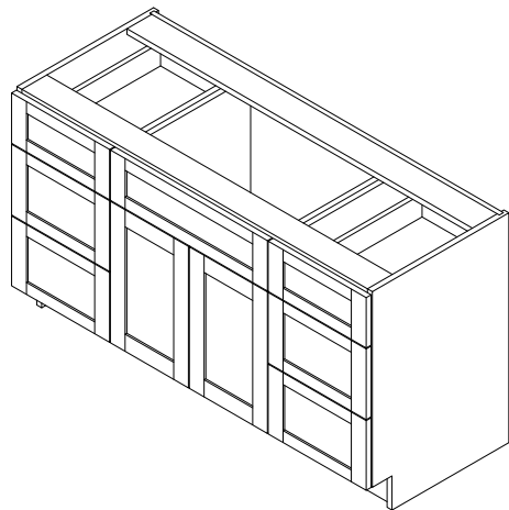
V6D 3 Standard Drawers each Side, 1 Fixed Drawer Front and Doors in Center
