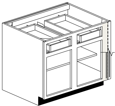
M22 Inside Extended Stiles (Straight, Fluted, or Applied Moulding)
