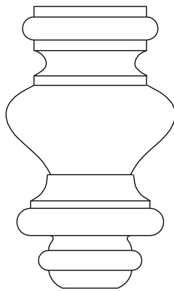
DBF03 Wood Bun Feet (3 3/4"W x 6 1/4"H)
