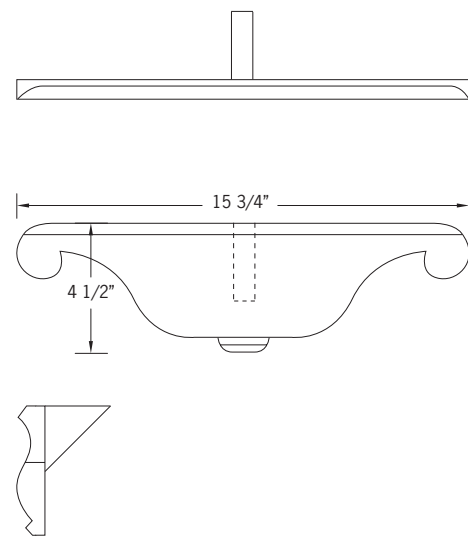
DBF12/B Wood Bun Feet (15 3/4"W x 4 1/2"H)
